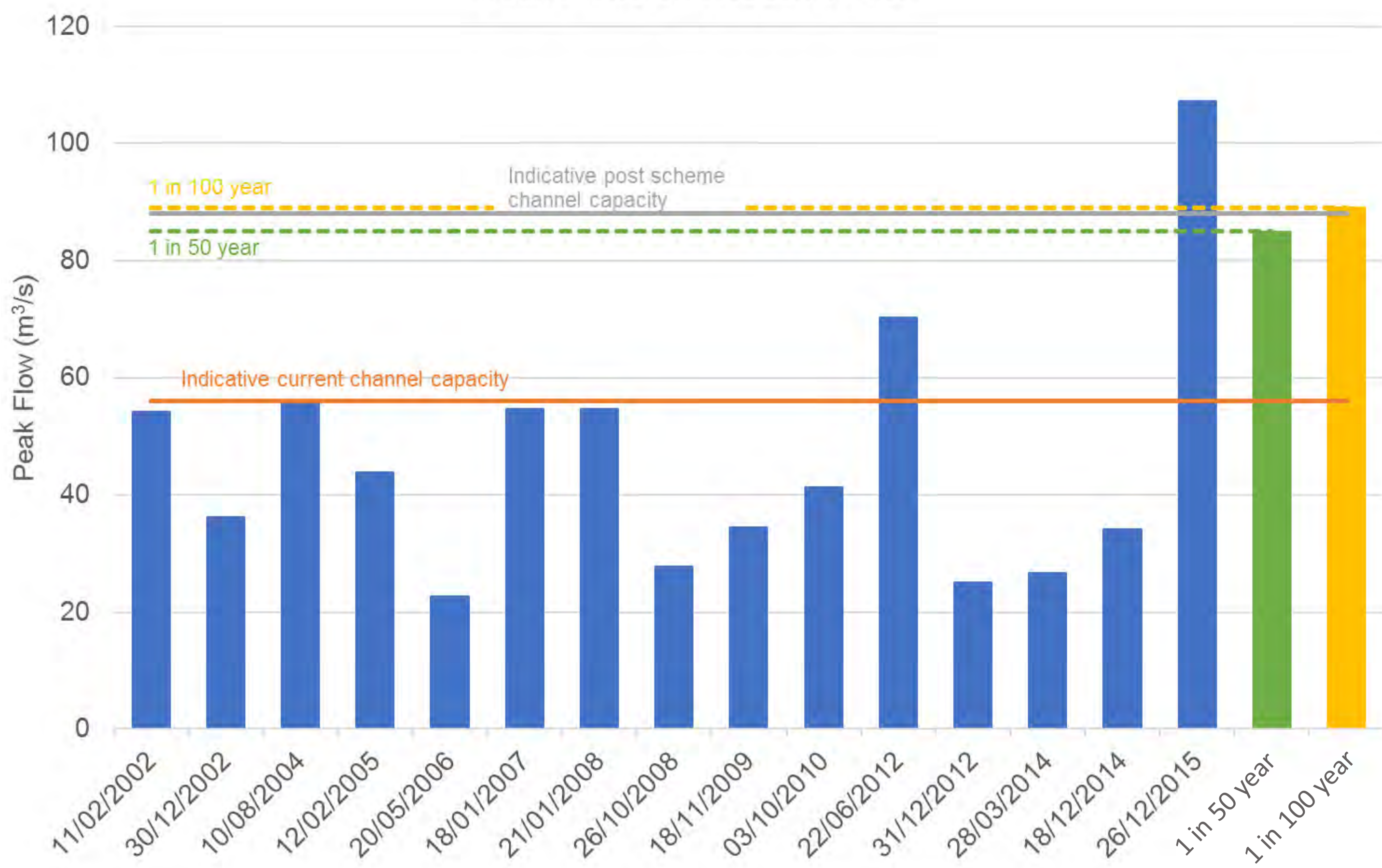
Peak Flows on Hebden Water
